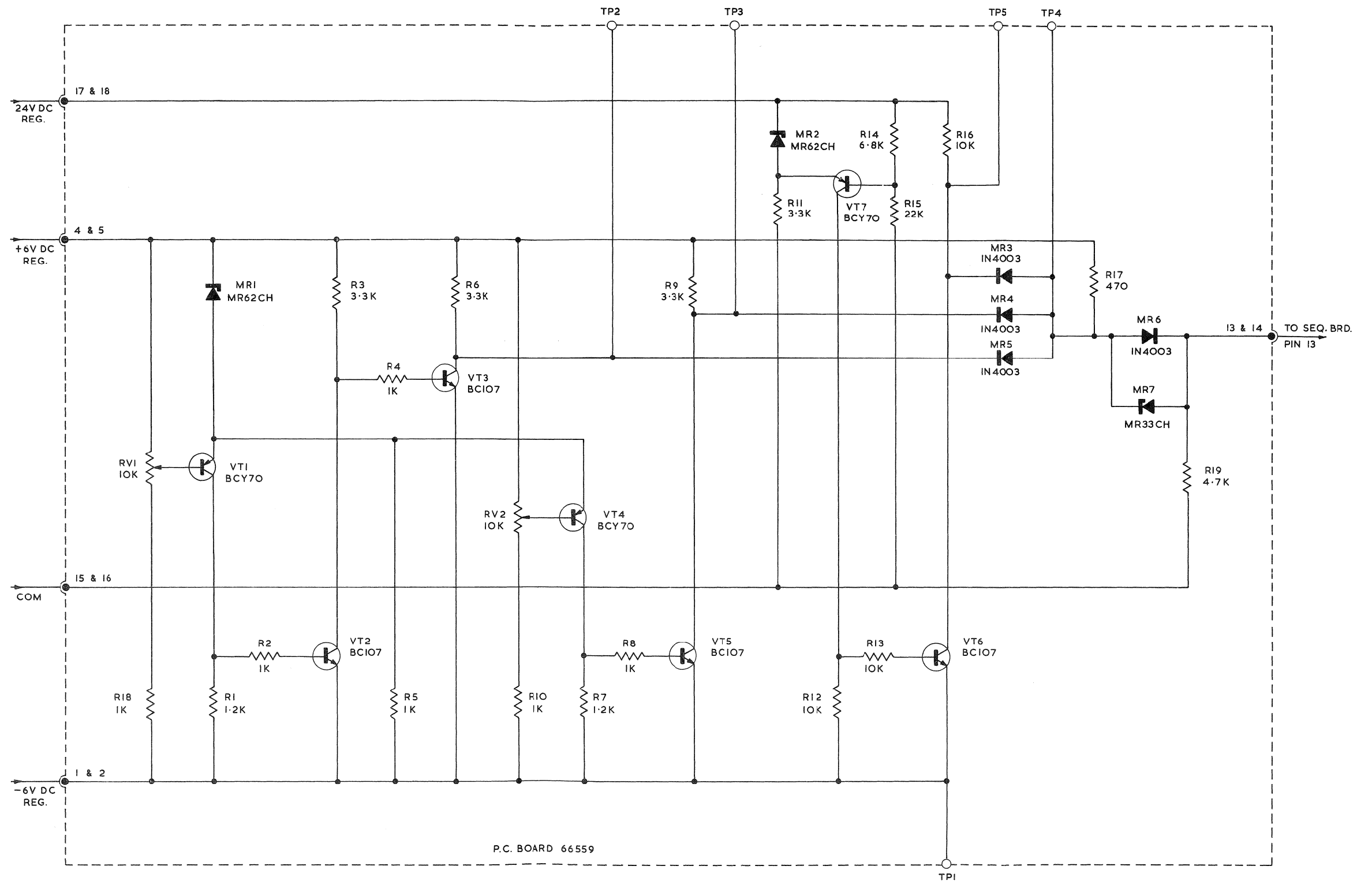
Figure 8-6 ±6 Volt Monitor Schematic
