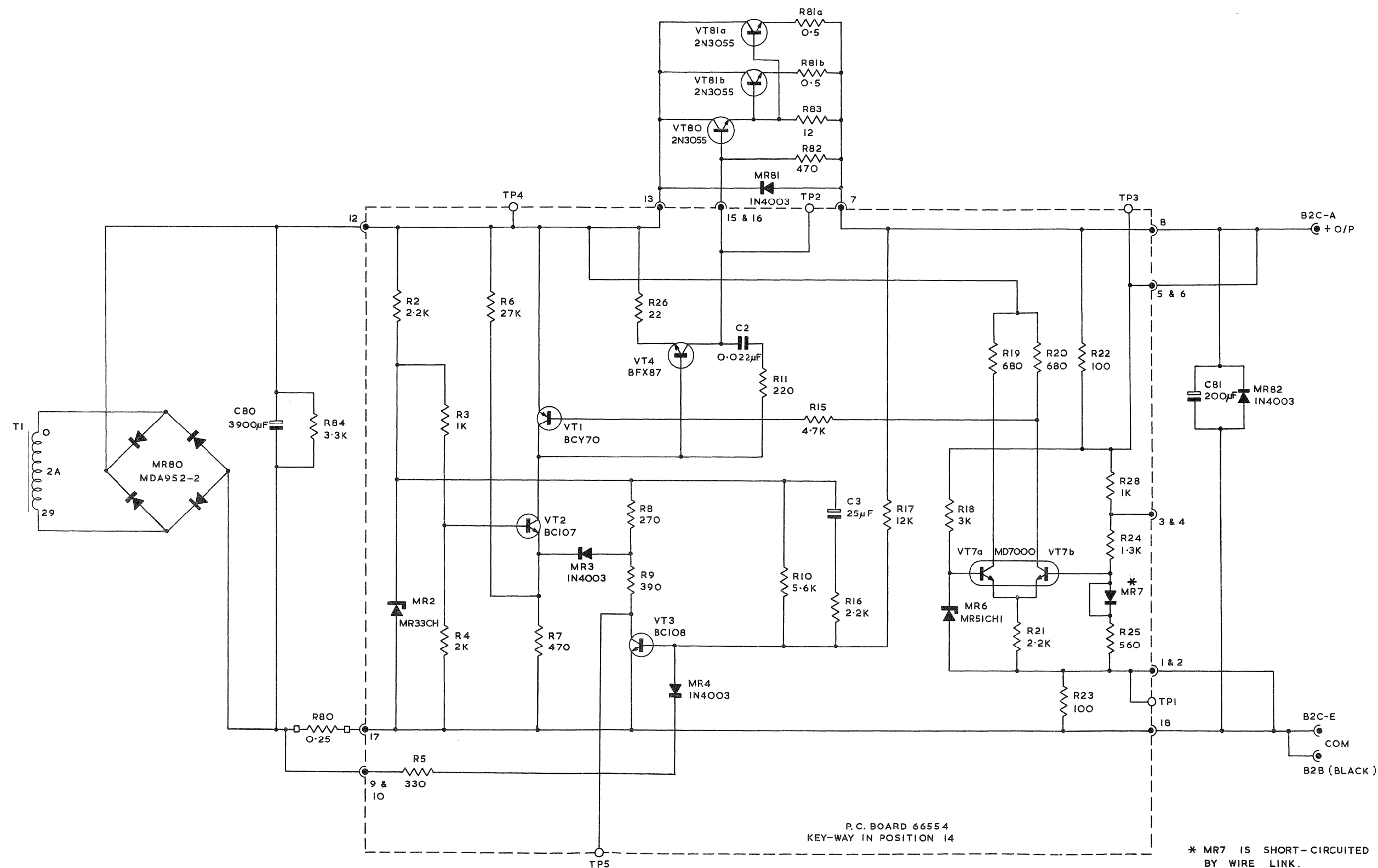
Figure 8-2 +24 Volt Series Regulator Schematic
